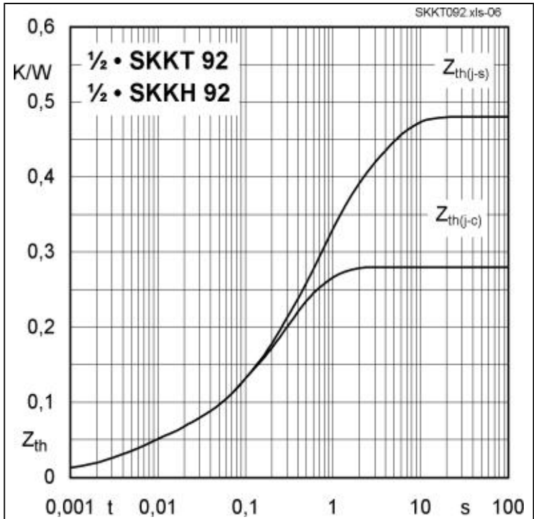
Fig. 6 Transient thermal impedance vs. time
