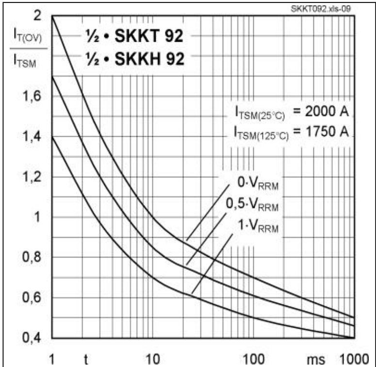
Fig. 8 Surge overload current vs. time
