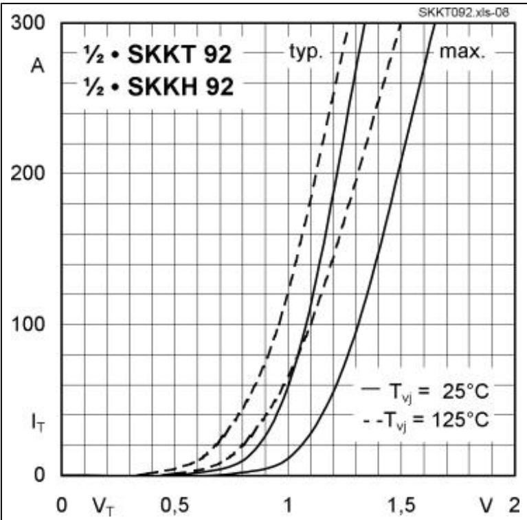
Fig. 7 On-state characteristics
